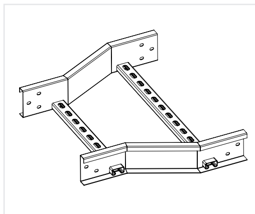
Centre Reducer KTCL 50 / 100 / 130 . CR / Width
