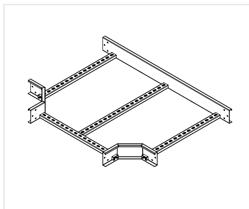
Equal Tee KTCL 50 / 100 / 130 . T / Width
