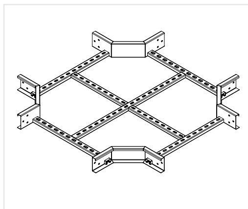
Crossover KTCL 50 / 100 / 130 . X / Width
