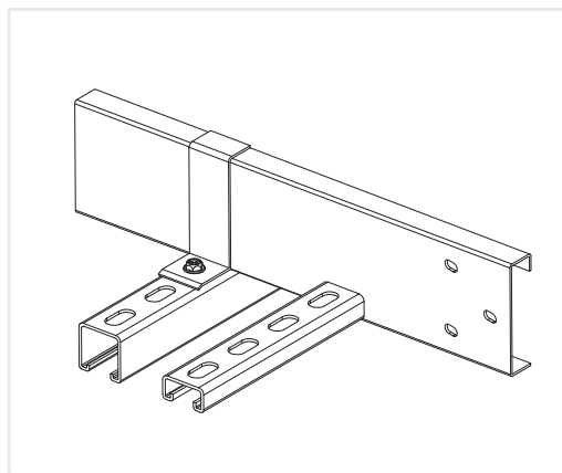
Hold Down Bracket KTCL 50 / 100 / 130 . HBD *M10 Fixing is required
