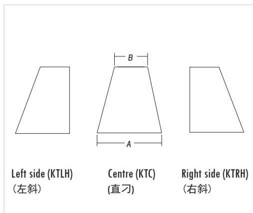
Reducer (直刁士) + / size A + / size B
