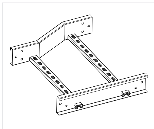
Right Hand Offset Reducer KTCL 50 / 100 / 130 . RHR / Width
