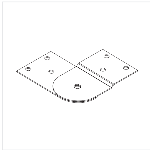
../VC Vertical Hinged Coupler KTCL 50 KTCL 100 / 130
