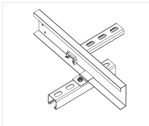
Ladder Clip KTCLC *M10 Fixing is required
