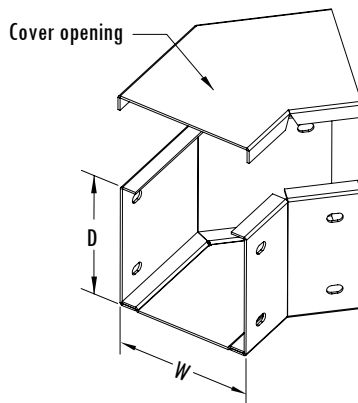
45 degree Front Opening Bend (45度 面曲) FB + / standard code
