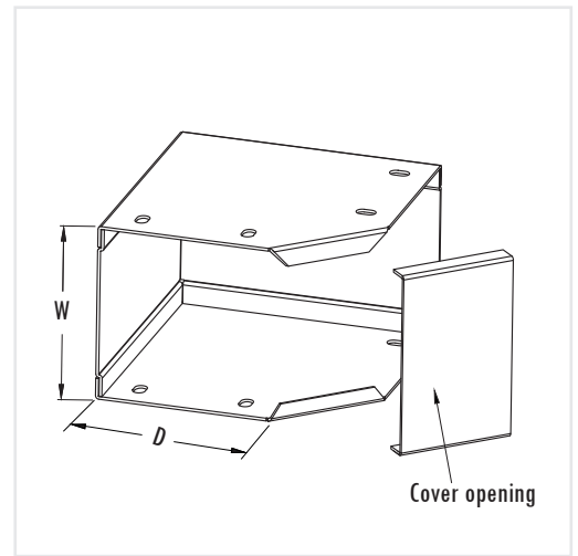
90 degree Internal Opening Bend (90度 內曲)
