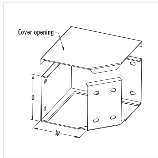
90 degree Front Opening Bend (90度 大面曲)
