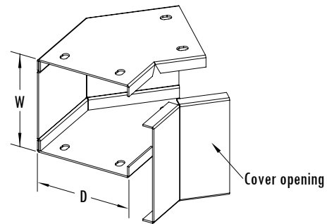
45 degree Internal Opening Bend (45度 內曲) FIB + / standard code
