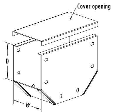
External Opening Tee (頂蓋T) ET + / standard code
