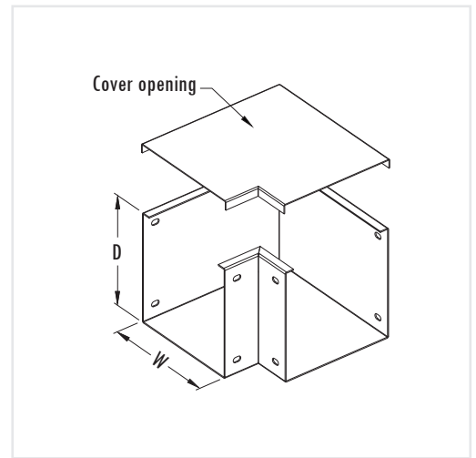
90 degree Front Opening Elbow (90度 直角面曲)
