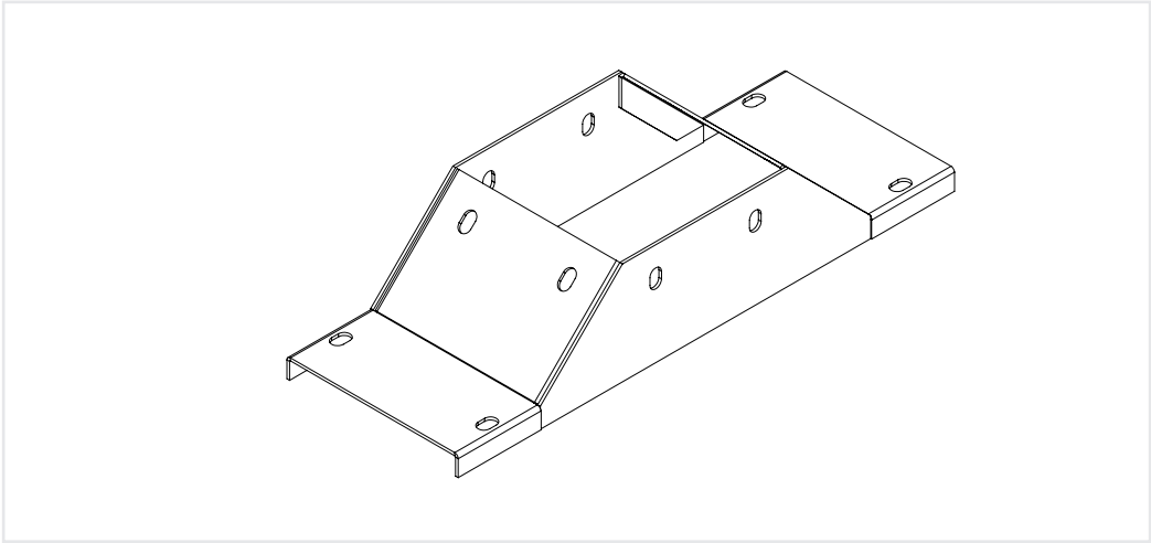
Cover Tee (直出蓋T) Remark: for 2 compartment Cover Tee: Standard Product Code + / 2
