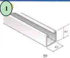
PLAIN CHANNEL - 3m
