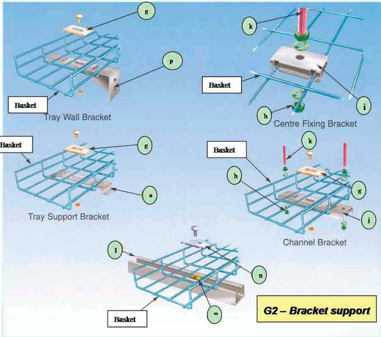
BRACKET FIXING KIT
